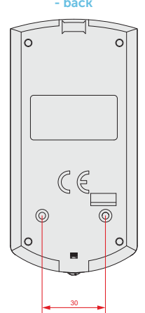
XIRP200H, XDTP200H, XDTP200HM, XTTP200H - back
