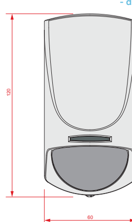
XIRP200H, XDTP200H, XDTP200HM, XTTP200H - dimensions
