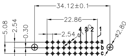
PCB LAYOUT(RECOMMENDED) (TOP VIEW TOL. :±0.05)
